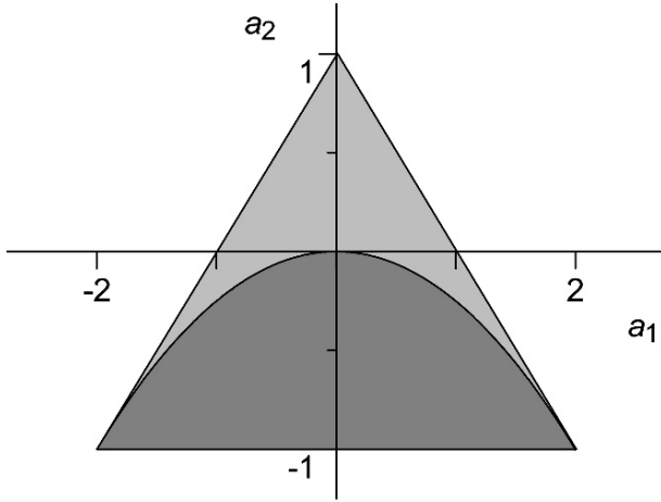
Figure 2.4. Regions of asymptotic stationarity for the AR(2) process (Eq. 2.14) (shaded). The region for complex roots (dark shaded), which allows quasi-periodic behaviour, lies below the parabolic, a_2 < -a_1^2/4 .
