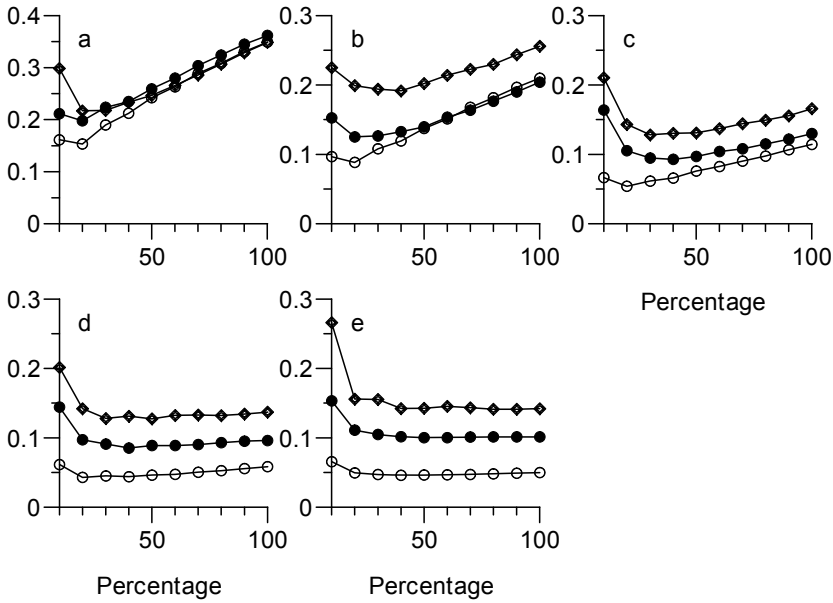
Figure 7.7. Monte Carlo study of synchrony Pearson's correlation coefficient for unequal timescales, dependence on percentage. a \tau_X = \tau_Y = 5 ; b \tau_X = \tau_Y = 10 ; c \tau_X = \tau_Y = 20 ; d \tau_X = \tau_Y = 50 ; e \tau_X = \tau_Y = 100 ; a–e wildly mixed unequal timescales and \rho_{XY} = 0.8 . See Fig. 7.4 as regards timescale and time series generation. Each panel shows for n = 100 (open diamonds), 200 (filled circles) and 1000 (open circles) the empirical \text{RMSE}_{\hat{r}_{XY\beta 100\%}} in dependence on the percentage (i.e., \beta ).
