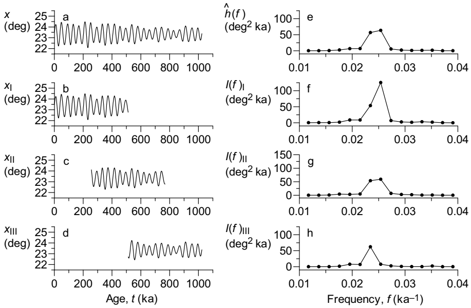
Figure 5.4. Welch's Overlapped Segment Averaging. a Time series of the obliquity of Earth's rotational axis over the past 1.024 Ma ( n = 1024, d(i) = d = 1 ka). The record was produced (Berger and Loutre 1991) by solving the astronomical, kinetic equations (many-body system). The record is segmented as follows: b segment I, points 1 to 512; c segment II, points 257 to 768; and d segment III, points 513 to 1024. The periodograms (Eq. 5.19) are calculated for segments I ( f ), II ( g ) and III ( h ). The average of the periodograms ( e ) has a maximum at T_{\text{period}} = 512/13 ka \approx 39.4 ka. Only a part of the frequency interval 0 to 1/2 ka ^{-1} is shown in e–h ; deg, degrees.
