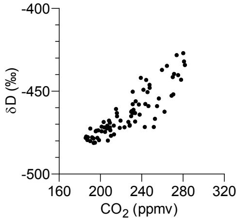
Figure 7.8. Vostok deuterium and \text{CO}_2 over the past 420 ka, correlation. Shown is the binned bivariate sample. The binned Pearson's correlation coefficient is \bar{r}_{XY} = 0.876 .
