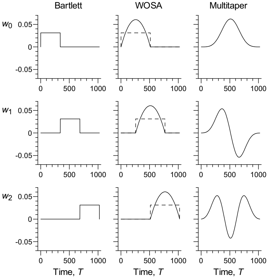
Figure 5.5. Tapers for spectral estimation. Shown are the functions w_k(T) , k = 0, \dots, K-1 , for averaging K = 3 (modified) periodograms, respectively eigenspectra; here 0 \leq T < 1024 and n = 1024 . The Bartlett type corresponds to non-overlapping and the WOSA type to (here) 50% overlapping segments. The WOSA type is shown with a uniform taper ( dashed lines ) and a normalized Welch taper ( solid lines ). The non-normalized Welch taper in continuous time is given by, for example, w'_0(T) = 1 - [(T - 256)/256]^2 for 0 \leq T \leq 512 ; the normalized Welch taper in discrete time by w_0(i) = w'_0(i)/\sqrt{\sum_{i=1}^n w'_0(i)^2} . The dpss multitaper functions have as additional parameter a resolution bandwidth of 2W = 4/(nd) ; that is, w_k(i) = v_k^{n,W}(i) ; for convenience of presentation these discrete functions are shown as continuous plots.
