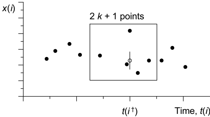
Figure 4.15. Outlier detection. The time point analysed for an outlier is t(i^\dagger) . The background or trend value is estimated as the median over 2k + 1 points inside a window, \hat{X}_{\text{trend}}(i^\dagger) = \widehat{M} \{X(i)\}_{i=i^\dagger-k}^{i^\dagger+k} ; the variability around that value is estimated as the median of absolute distances to the median (MAD) over the 2k + 1 points, \hat{S}(i^\dagger) = \widehat{M} \left\{ \left| X(j) - \widehat{M} \{X(i)\}_{i=i^\dagger-k}^{i^\dagger+k} \right| \right\}_{j=i^\dagger-k}^{i^\dagger+k} . In the example, the data points are shown as filled symbols , k = 2 and the background \pm variability estimate is shown as open symbol with vertical bars . Adopting a (likely too low) threshold detection parameter of z = 2 would make t(i^\dagger) a detected extreme because x(i^\dagger) is more than 2\hat{S}(i^\dagger) away from \hat{X}_{\text{trend}}(i^\dagger) ; a threshold detection parameter of z = 3.5 would reject the point as an extreme. For detecting outliers in the whole series, the window is pointwise shifted. A simple solution for outlier detection near the interval bounds ( i \rightarrow 1, i \rightarrow n ) is to extrapolate background and variability there.
