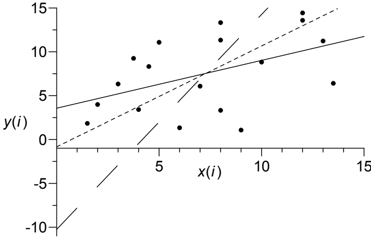
Figure 8.2. Linear errors-in-variables regression model, WLSXY and OLS estimations. The \{x(i), y(i)\}_{i=1}^n are overtaken from Fig. 8.1c. The OLS fit of X on Y (solid line) has a slope of \hat{\beta}_1 = 0.55 , the OLS fit of Y on X (long-dashed line) has 1/\hat{\beta}_1' = 2.45 and the WLSXY fit of X on Y (short-dashed line) has \hat{\beta}_1 = 1.15 . (The model for the regression of Y on X is X(i) = \beta_0' + \beta_1'Y(i) + S_X \cdot X_{\text{noise}}(i) .)
