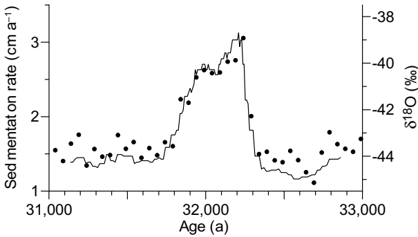
Figure 4.9. Onset of Dansgaard-Oeschger event 5, NGRIP ice core: sedimentation rate (solid line) and \delta^{18}\text{O} (dots) variations. ( \delta^{18}\text{O} data from North Greenland Ice Core Project members 2004 .)
