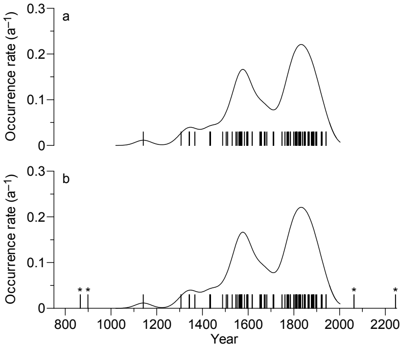
Figure 6.4. Elbe winter floods, pseudodata generation. The heavy events (magnitudes 2–3) are taken from the complete record (Fig. 1.1) and plotted (a, b) as bars ( m = 73 ). The “twopoint” rule is used to generate four pseudodata points (b, asterisks ) outside the observation interval. Occurrence rates are estimated with h = 35 a, and without (a m^\dagger = 73 ) or with (b m^\dagger = 77 ) pseudodata.
