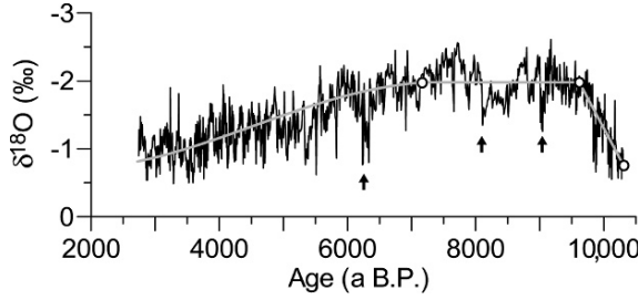
Figure 4.18. Trend estimation for the \delta^{18}\text{O} record from stalagmite Q5. A combination of a portion of a ramp in the early part and a sinusoid in the late part was fitted (OLS) as trend (grey line) to the time series (black line). Choice of the sinusoid is motivated by the observation that Holocene changes in local solar insolation, induced by Earth orbital changes, influenced monsoonal rainfall amounts (Fleitmann et al. 2003). The change-point estimates (open circles) with bootstrap standard errors (SB resampling, B = 2000 , time errors from statistical and dating (Fleitmann et al. 2003) uncertainties via Gaussian error propagation) are (10,300 a (fixed), -0.77 \pm 0.08\text{‰} ), ( 9617 \pm 89 a, -1.98 \pm 0.03\text{‰} ) and ( 7200 \pm 400 a, -1.98\text{‰} ). The change at 9617 a occurred, within error bars, simultaneously with a similar change in northern temperatures, as indicated by \delta^{18}\text{O} variations in the GRIP ice core (Greenland), indicating a potential influence of northern glacial boundary conditions on monsoon climate (Fleitmann et al. 2003). The sinusoid was fitted by linear OLS regression (e.g., replace \beta_1 T(i) by \beta_1 \sin(T(i)) ). Climate extremes detection (Section 4.3.3) found three pronounced dry extremes (arrows): a longer-lasting event at \sim 8.2 ka and other at \sim 9.2 and \sim 6.3 ka.
